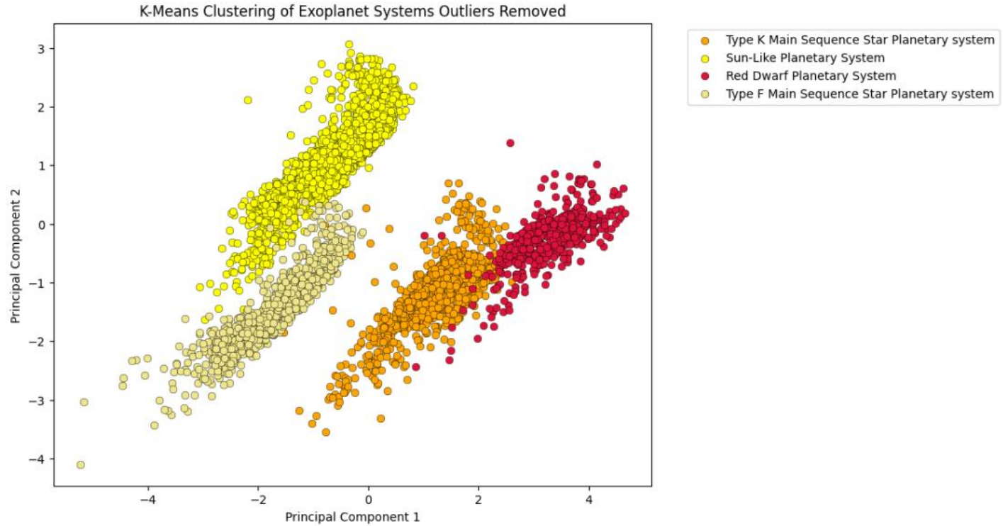
Figure 20: Graph shows the 4 clusters identified by the K-Means Cluster model for all confirmed exoplanets with 535 outlier exoplanets removed due to anomalous features present.
