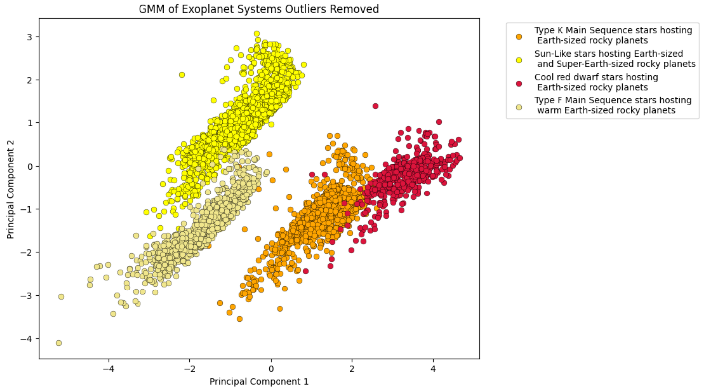
Figure 21: Graph shows the 4 clusters identified by the GMM model for all confirmed exoplanets with 535 outlier exoplanets removed due to anomalous features present.
